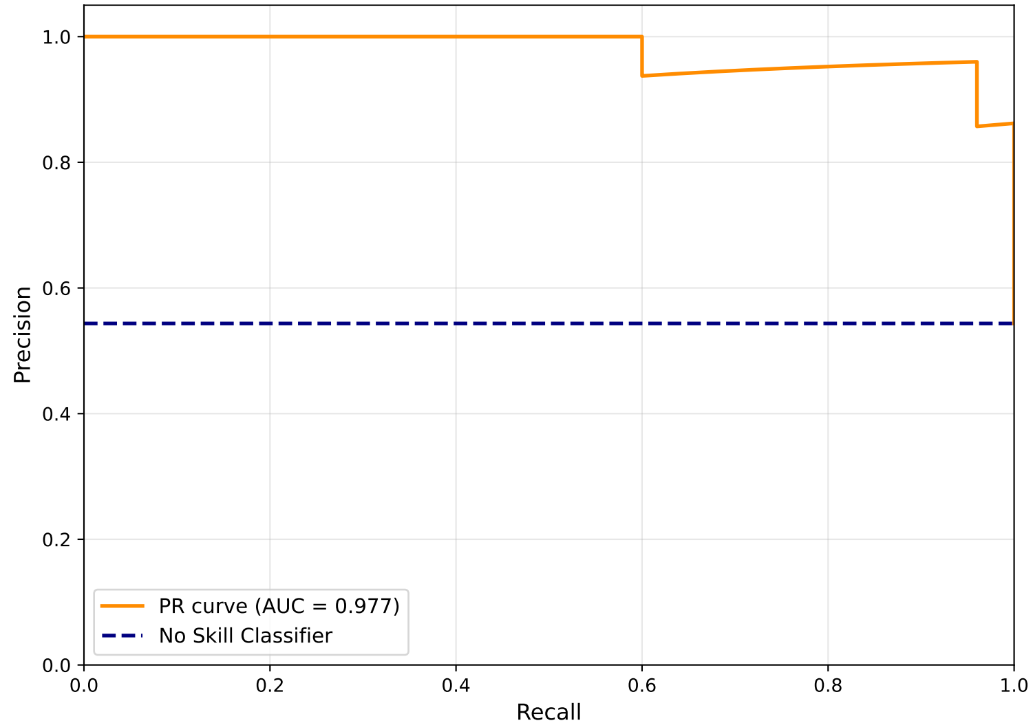
Precision-Recall Curve for Stacking Ensemble
